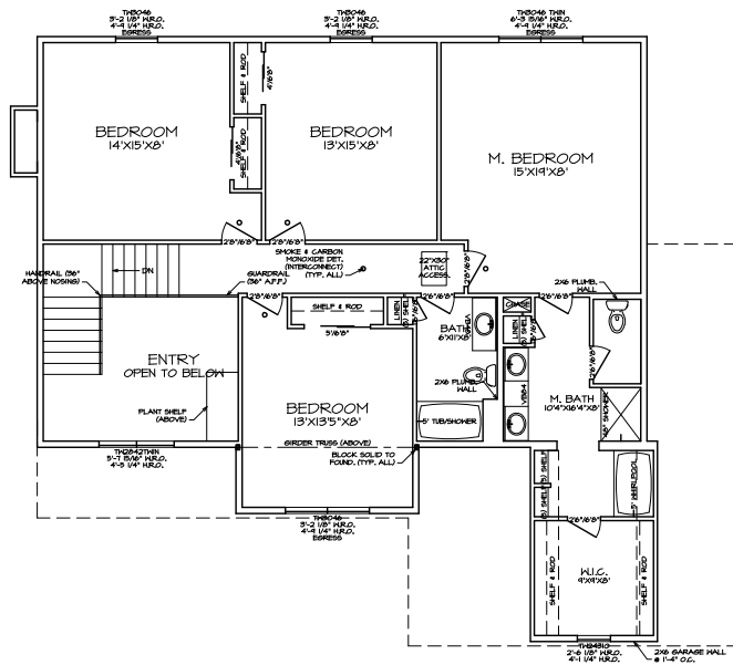
SECOND FLOOR PLAN A-5 SCALE: 1/4"=1'-0"
